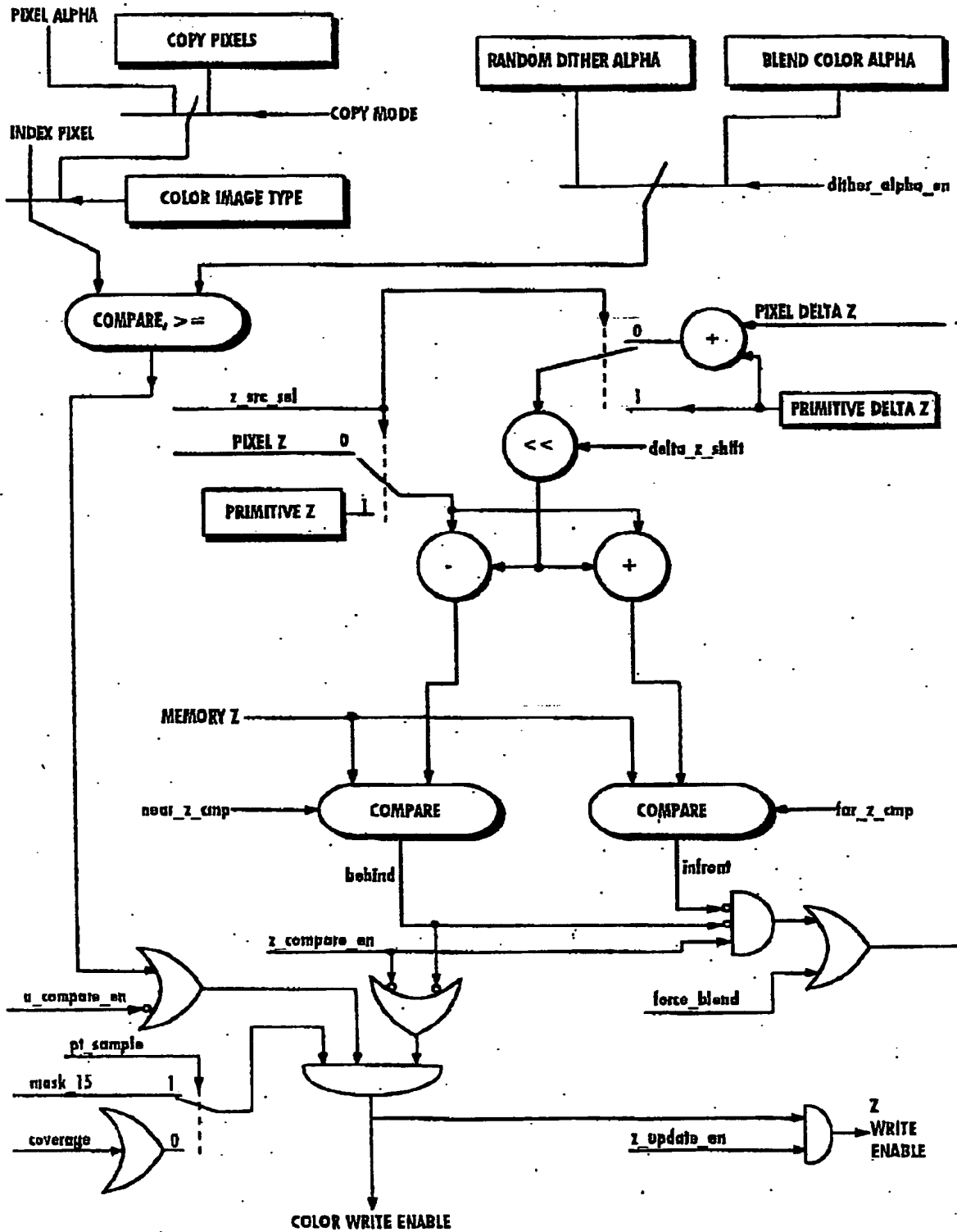
Fig. 33A WRITE ENABLE GENERATION
